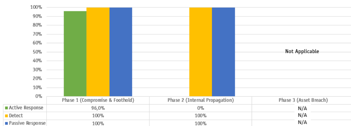
Figure 3 — Active vs Passive Response of Cisco Secure Endpoint Essentials
