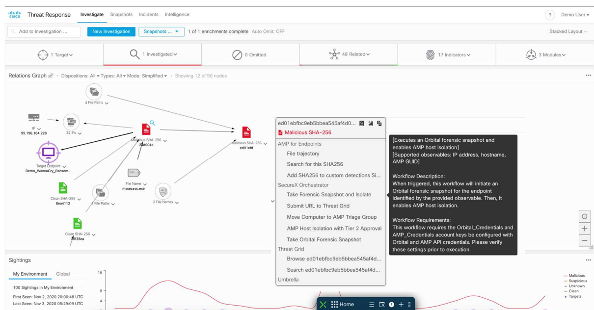
Cisco Secure Endpoint's SecureX Threat Response
