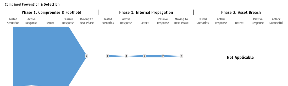
Figure 4 — EPR Efficacy per Phase of Cisco Secure Endpoint Essentials
