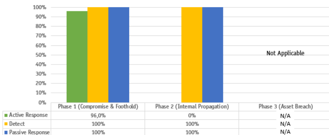
Figure 3 — Active vs Passive Response of ESET PROTECT Enterprise
