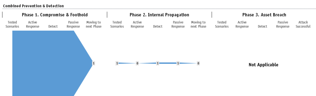
Figure 4 — EPR Efficacy per Phase of F-Secure Elements EDR and EPP for Computers
